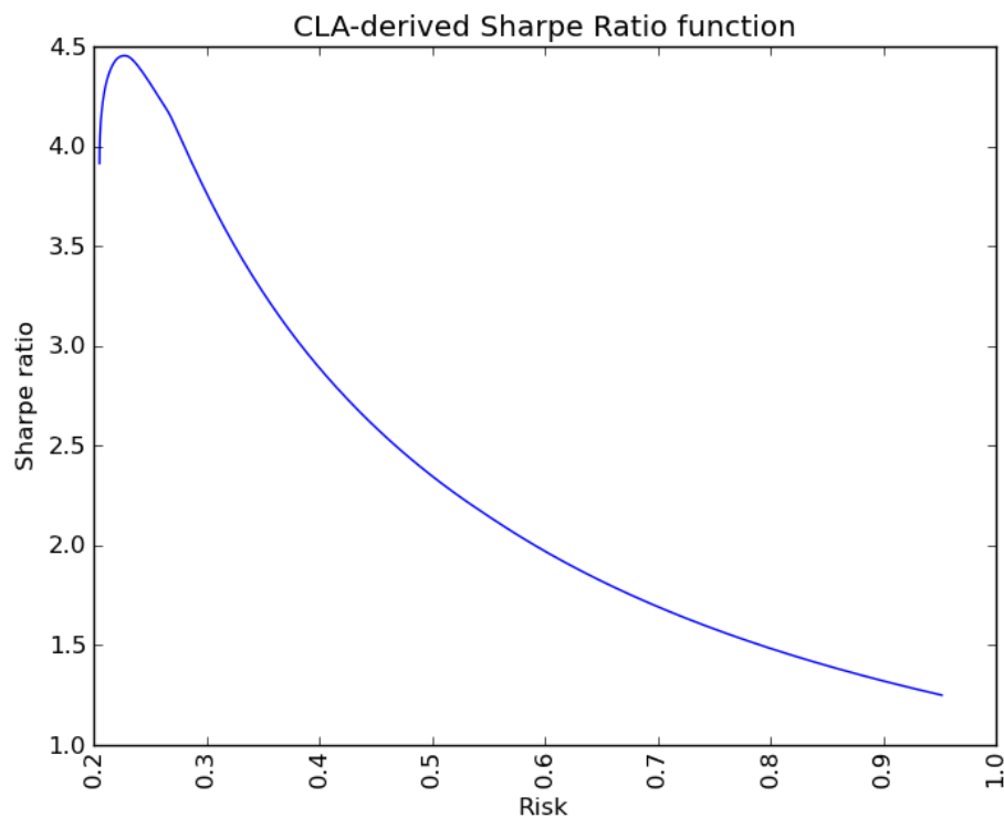
Figure 2. Sharpe ratio as a function of risk
